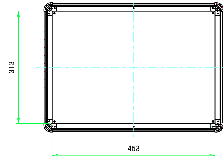
C-C (1:6)
